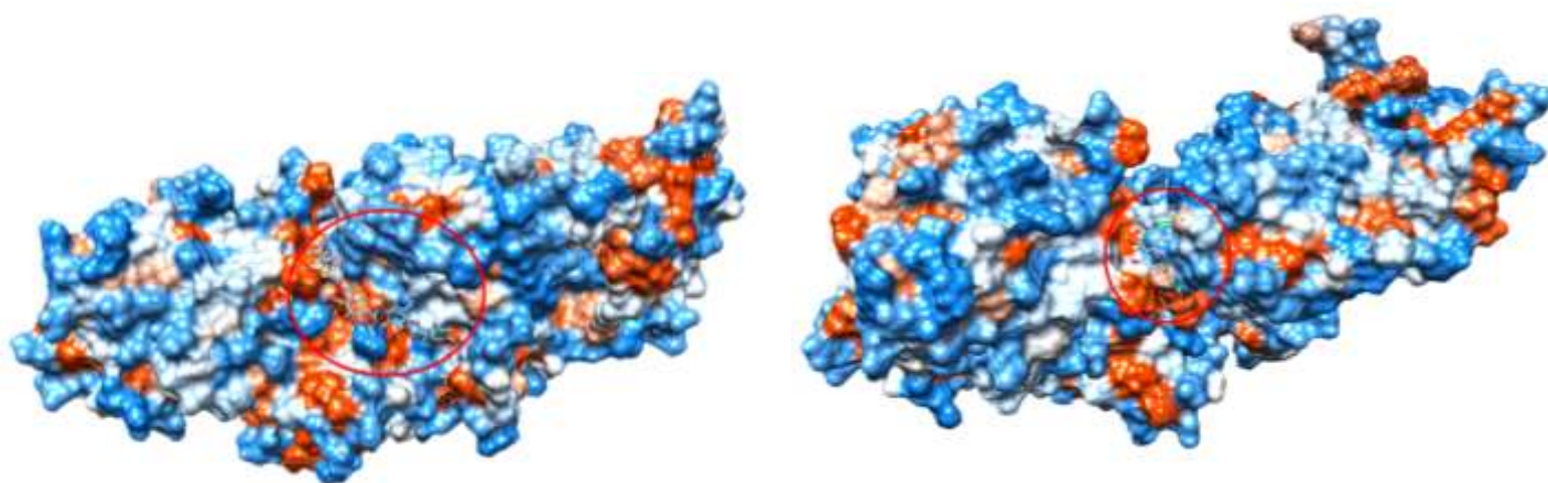
Figure 11. Three-dimensional illustration of the 3PP0 - Lapatinib (A) and 3PP0 - meletin (B) using the molecular surface
