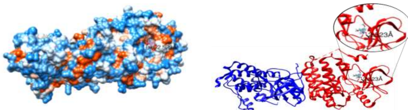
Figure 9. Three-dimensional illustration of the 3PP0 - \alpha -Linolenic complex using the molecular surface (A) and the ribbon model (B).
