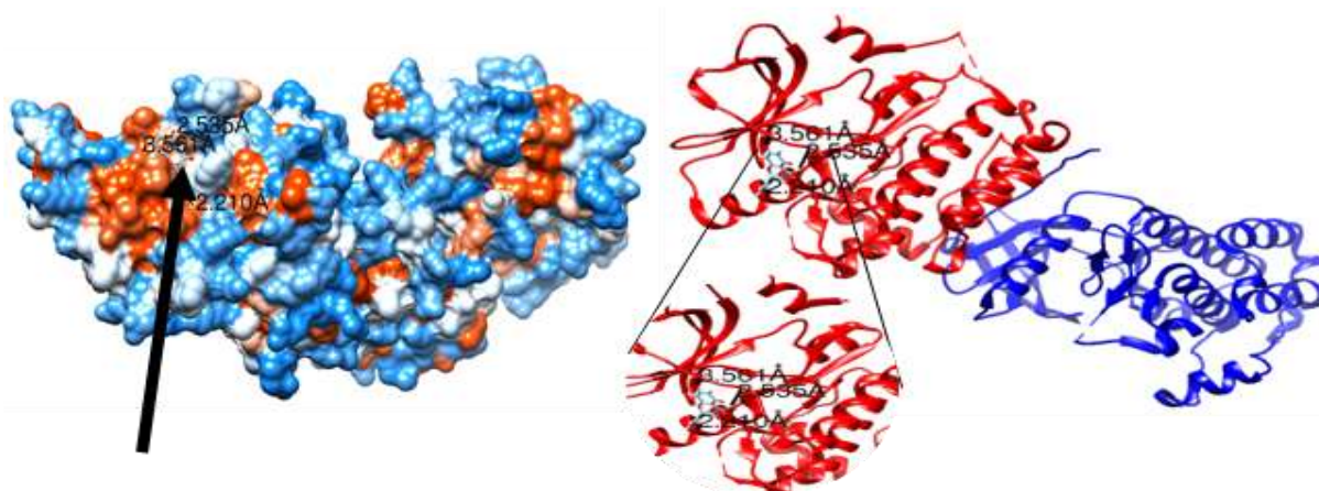
Figure 10. Three-dimensional illustration of the 3PP0 - Kaempferol complex using the molecular surface (A) and the ribbon model (B).
