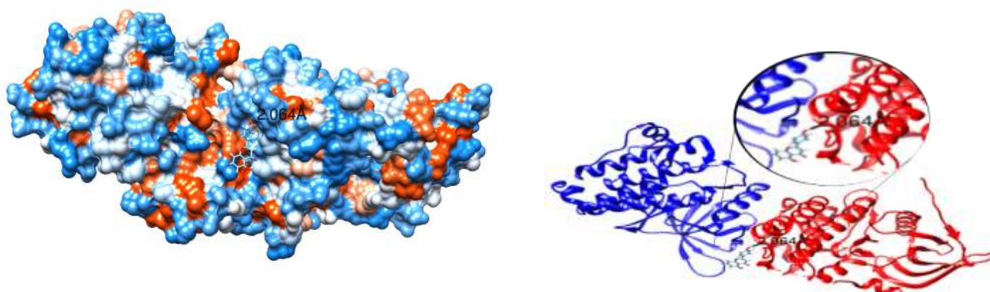
Figure 7. Three-dimensional illustration of the 3PP0- Apigenin complex using the molecular surface (A) and the ribbon model (B).
