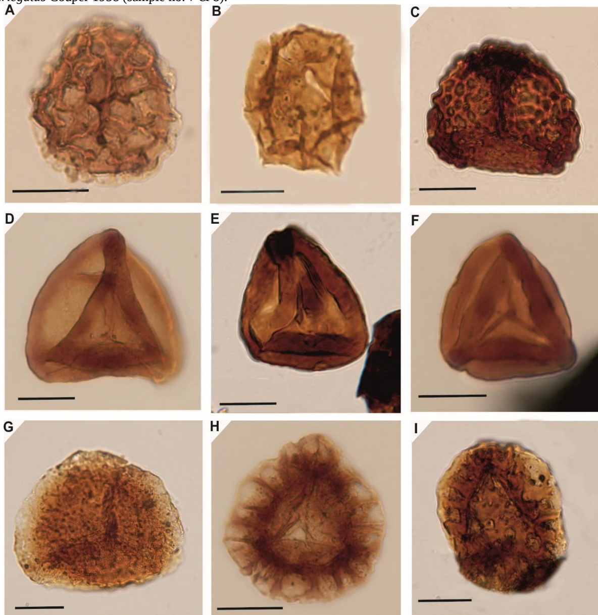
Fig. 9. Spores from upper Bajocian strata of the Binalud Mountains (scale bars=20µm; proximal foci for all samples except for sample B, which show median focus). A, Retitriletes austroclavatidites (Cookson 1953) Döring, Krutzsch, Mai & Schulz 1963 (sample no. 8); B, Retitriletes polygonatus Hashemi-Yazdi, Sajjadi & Dehbozorgi 2015 (sample no. 5); C, Ischyosporites crateris Balme 1957 (sample no. 5); D & E, Gleicheniidites senonicus (Ross 1949) emend. Skarby 1964 (sample no. 6 & -1); F, Kyrtomisporis laevigatus Mädlar 1964 (sample no. 7); G, Perotrilites granulatus Couper 1953 (sample no. 3); H, Limboisporites antiquus (de Jersey 1964) de Jersey & Raine 1990 (sample no. 8); I, Limboisporites lundbladii Nilsson 1958 (sample no. -1).
