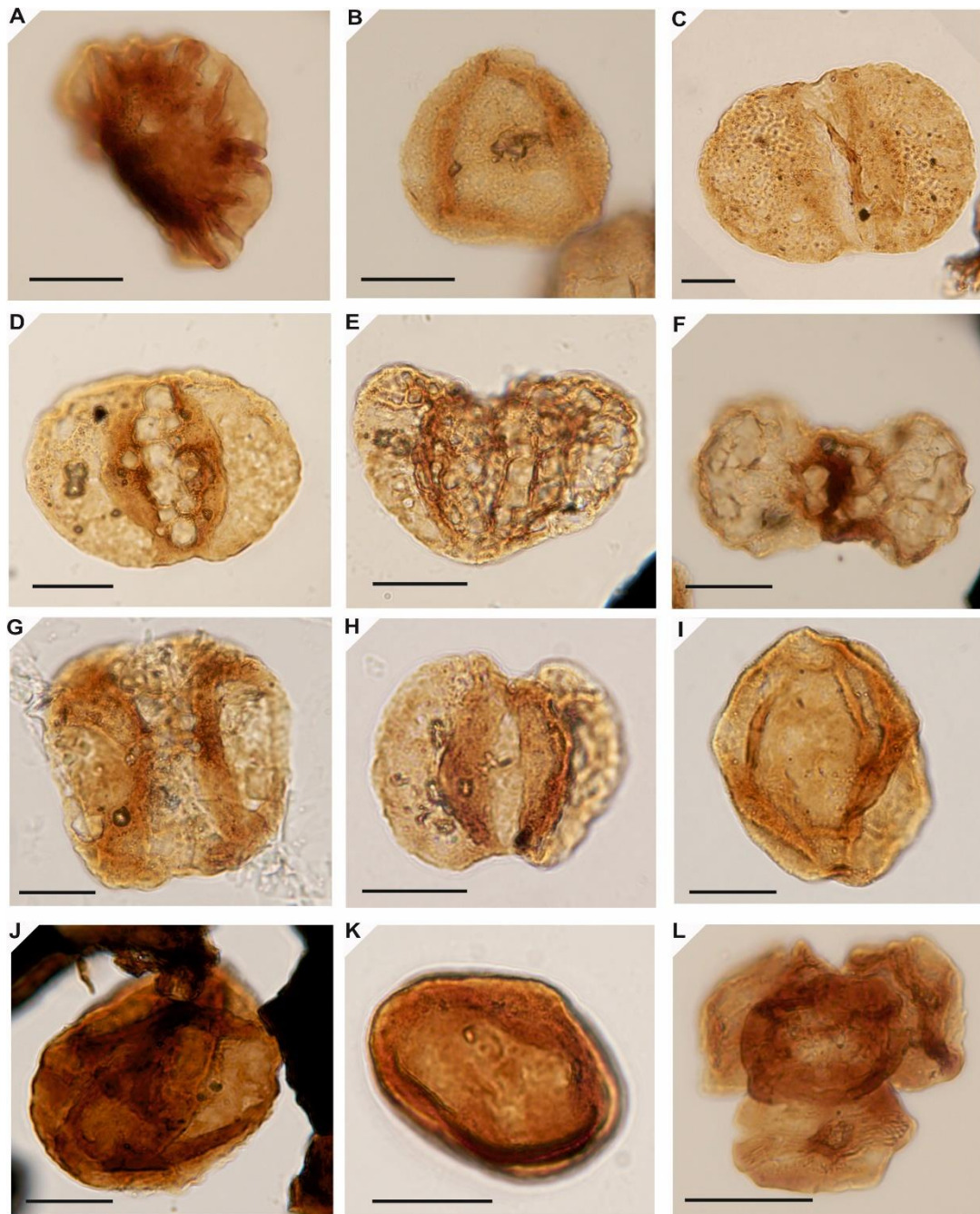
Fig. 10. Pollen grains from upper Bajocian strata of the Binalud Mountains (scale bars=20µm). A, Callialasporites dampieri (Balme 1957) Sukh Dev 1961 (sample no. 8; polar view); B, Callialasporites turbatus (Balme 1957) Schulz 1967 (sample no. 7, polar view); C, Alisporites grandis (Cookson 1953) Dettmann 1963 (sample no. 5; median focus); D, Alisporites australis de Jersey 1962 (sample no. 2; median focus); E, Indusiisporites parvisaccatus (de Jersey 1959) de Jersey 1963 (sample no. 4; median focus); F, Platysaccus queenslandi de Jersey 1962 (sample no. 7; distal focus);
