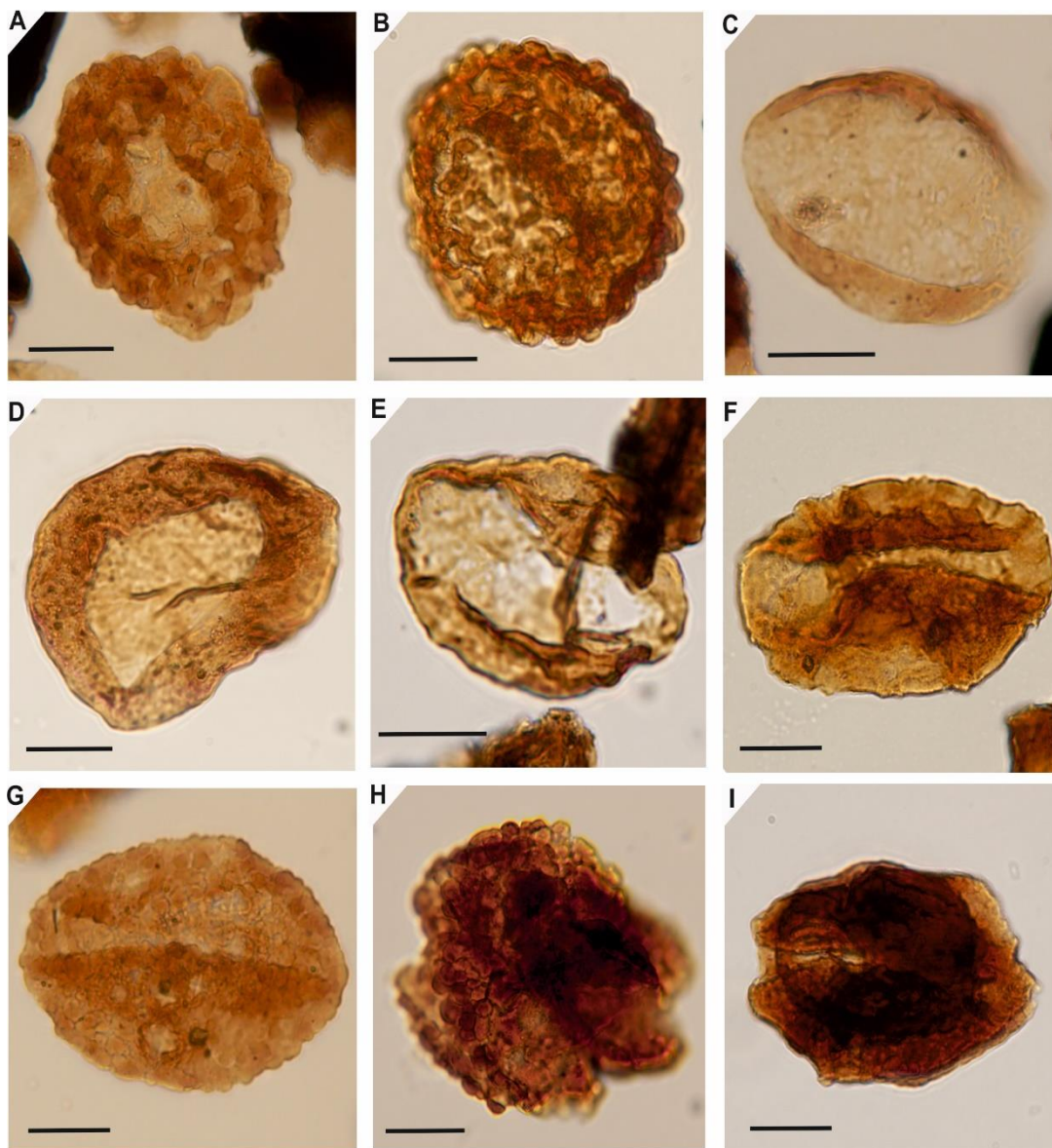
Fig. 11. Pollen grains from upper Bajocian strata of the Binalud Mountains (scale bars=20 \mu m; median foci for all samples). A & B, Cerebropollenites macroverrucosus (Thiergart 1949) Schulz 1967 (sample no. 7 & 3); C & D, Chasmatosporites apertus (Rogalska 1954) Nilsson 1958 (sample no. 7 & 2); E, Chasmatosporites major Nilsson 1958 (sample no. -1); F, Cycadopites crassimarginis (de Jersey 1959) de Jersey 1964 (sample no. -1); G, Cycadopites granulatus (de Jersey 1959) de Jersey 1964 (sample no. 7); H & I, Ricciisporites tuberculatus Lundblad 1954 (sample no. 1 & 3).
