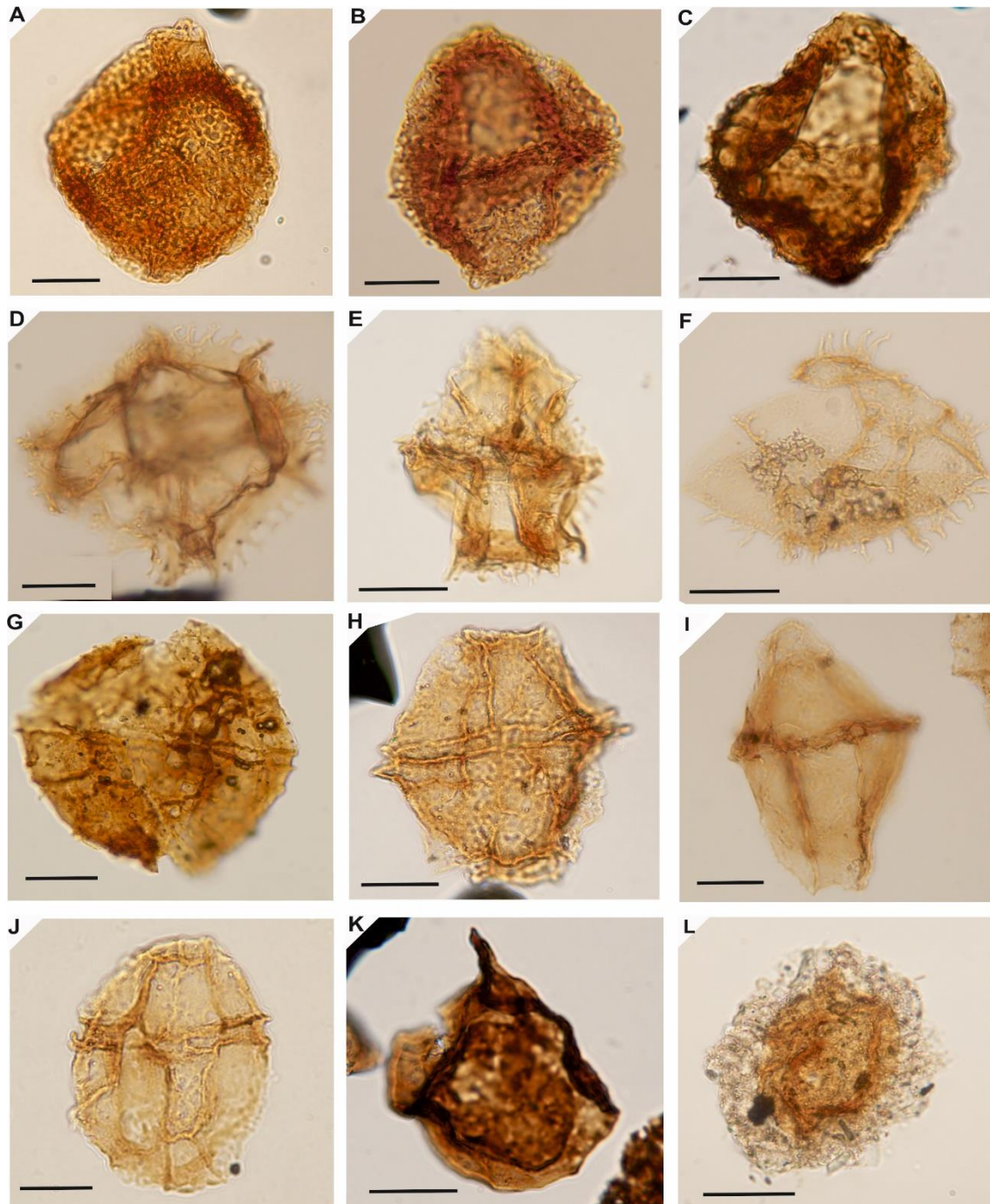
Fig. 4. Dinoflagellate cysts from upper Bajocian of the Binalud Mountains (scale bars=20 \mu m). A, Aldorfia alдорфensis (Gocht 1970) Stover & Evitt 1978 (sample no. 3); B & C, Cribroperidinium crispum (Wetzel 1967) Fenton 1981 (sample no. 1 & -1); D, Dichadogonyaulax combazii Dupin 1968 (sample no. 7); E, Ctenidodinium continuum Gocht 1970 (sample no. 1); F, Ctenidodinium sellwoodii (Sarjeant 1975) Stover & Evitt 1978 (sample no. 8); G, Meiourogonyaulax caytonensis (Sarjeant 1959) Sarjeant 1969 (sample no. -1); H, Meiourogonyaulax valensii Sarjeant 1966 (sample no. 5); I, Tubotuberella dangeardii (Sarjeant 1968) Stover & Evitt 1978 (sample no. 7); J,
