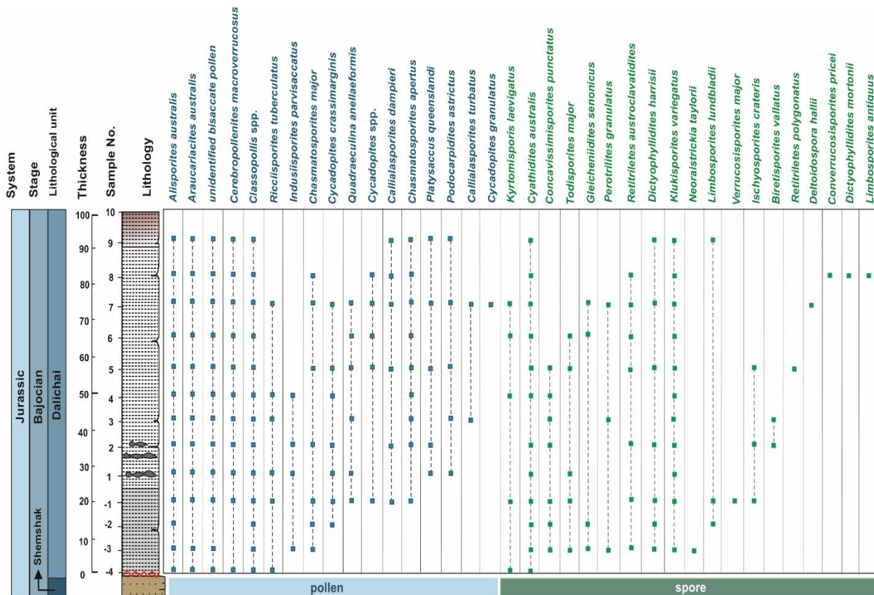
Fig. 7. Distribution of the pollen grains and spores in the upper Bajocian strata of the Dalichai Formation.
