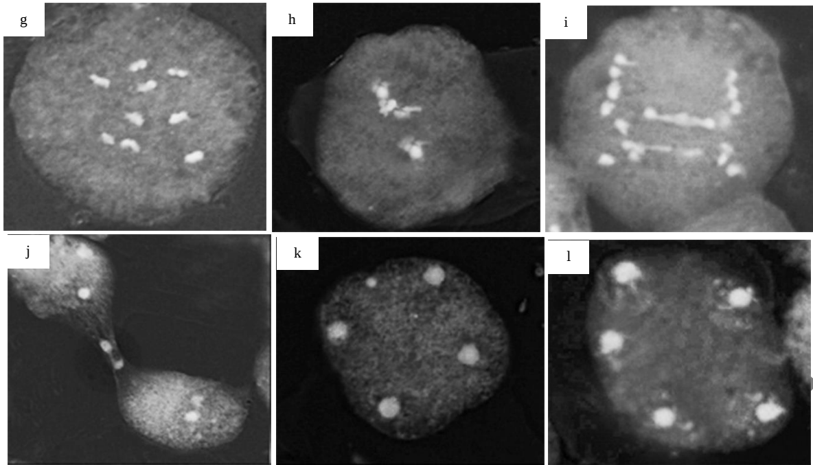
Fig. 1 Chromosomal aberrations at different stages of meiosis in N. racemosa (a-f) and N. pungens (g-l). a) Dyad with 9 bivalents. b) Chromosome stickiness. c) Premature chromosome separation. d) Laggard. e) Cytomixis in dyad. f) Tripolar. g) Dyad with 9 bivalents. h) Chromosome stickiness. i) Bridge. j) Cytomixis during telophase I. k) Micronucleus at telophase II. l) Pentapolar.
