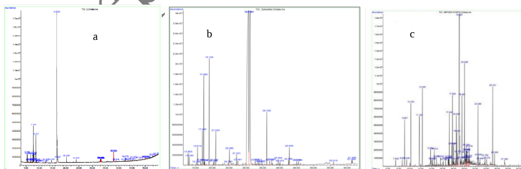
Fig. 8 GC-MS chromatogram of Thymus daenensis (a), Satureja bakhtiatica (b), and Carum carvi (c)
